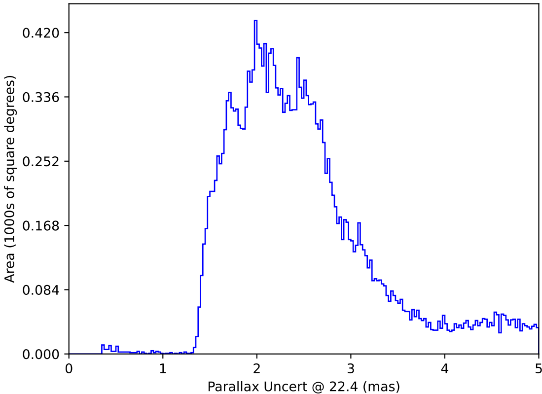
too_elab_r8_d3_giz_v3.4_10yrs All sky: Parallax Uncert @ 22.4
