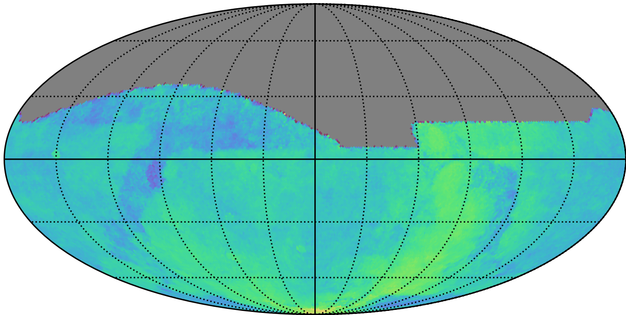
too_elab_r8_d3_giz_v3.4_10yrs All sky: Parallax Coverage @ 24.0
