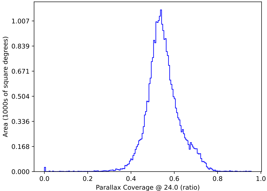
too_elab_r8_d3_giz_v3.4_10yrs All sky: Parallax Coverage @ 24.0
