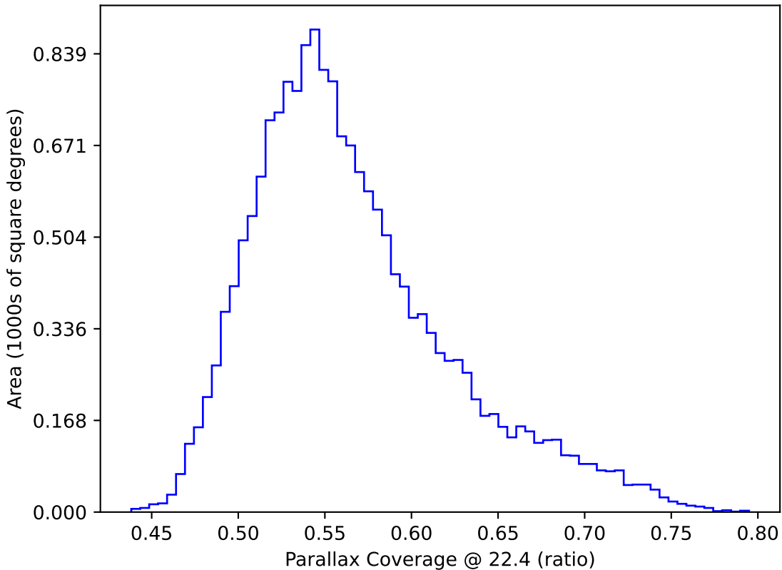
too_elab_r8_d3_giz_v3.4_10yrs WFD: Parallax Coverage @ 22.4
