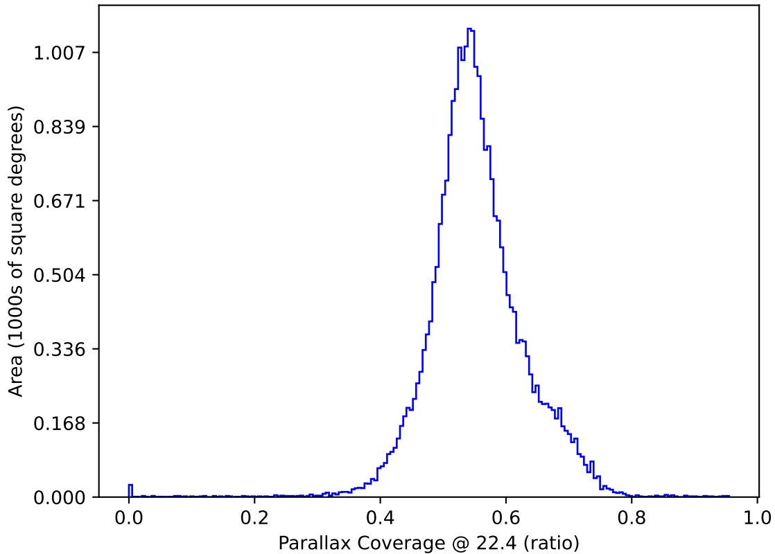
too_elab_r8_d3_giz_v3.4_10yrs All sky: Parallax Coverage @ 22.4
