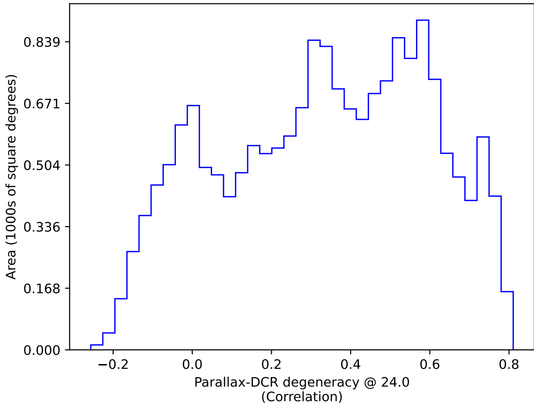
too_elab_r8_d3_giz_v3.4_10yrs WFD: Parallax-DCR degeneracy @ 24.0
