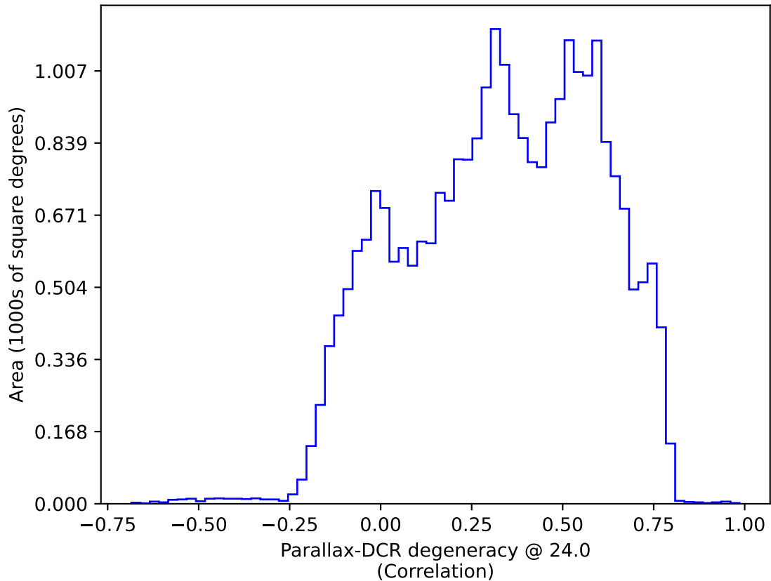
too_elab_r8_d3_giz_v3.4_10yrs All sky: Parallax-DCR degeneracy @ 24.0
