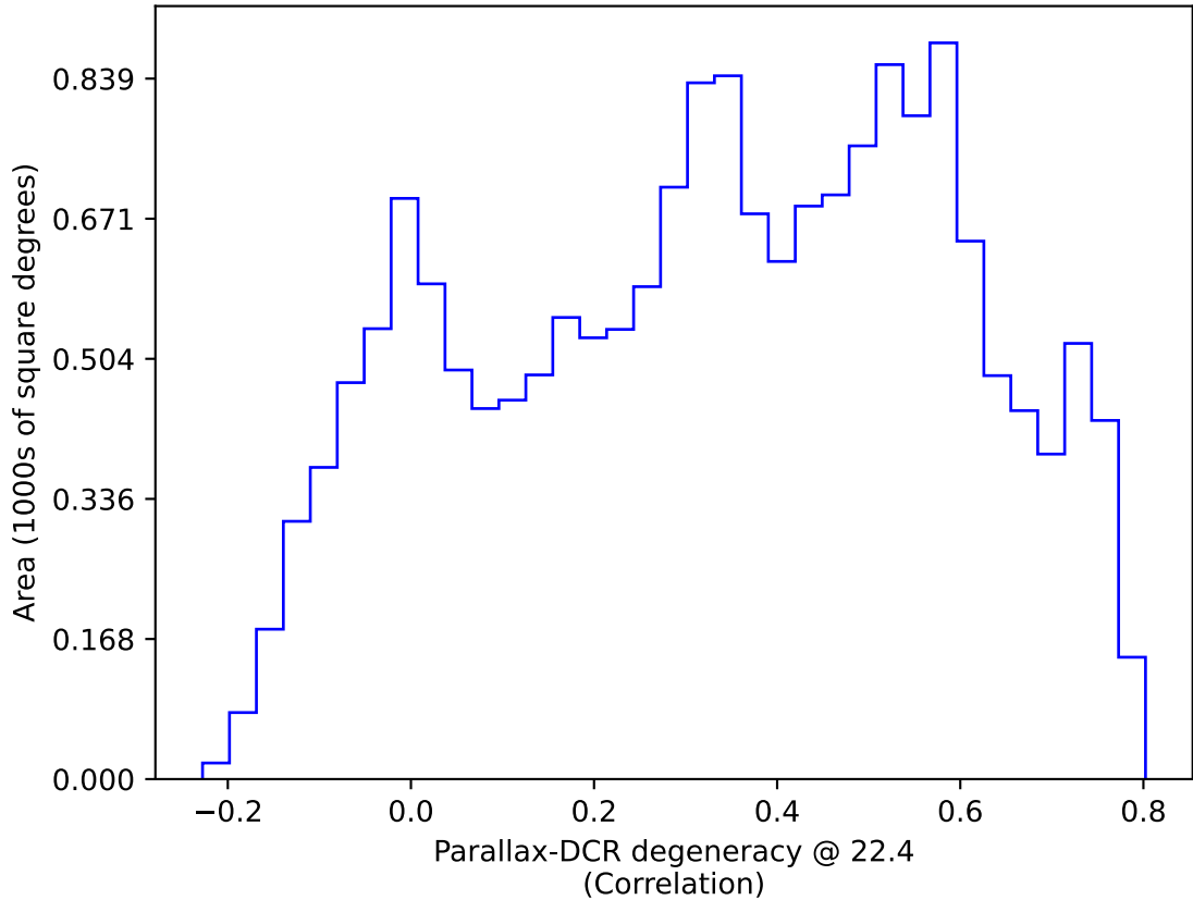
too_elab_r8_d3_giz_v3.4_10yrs WFD: Parallax-DCR degeneracy @ 22.4
