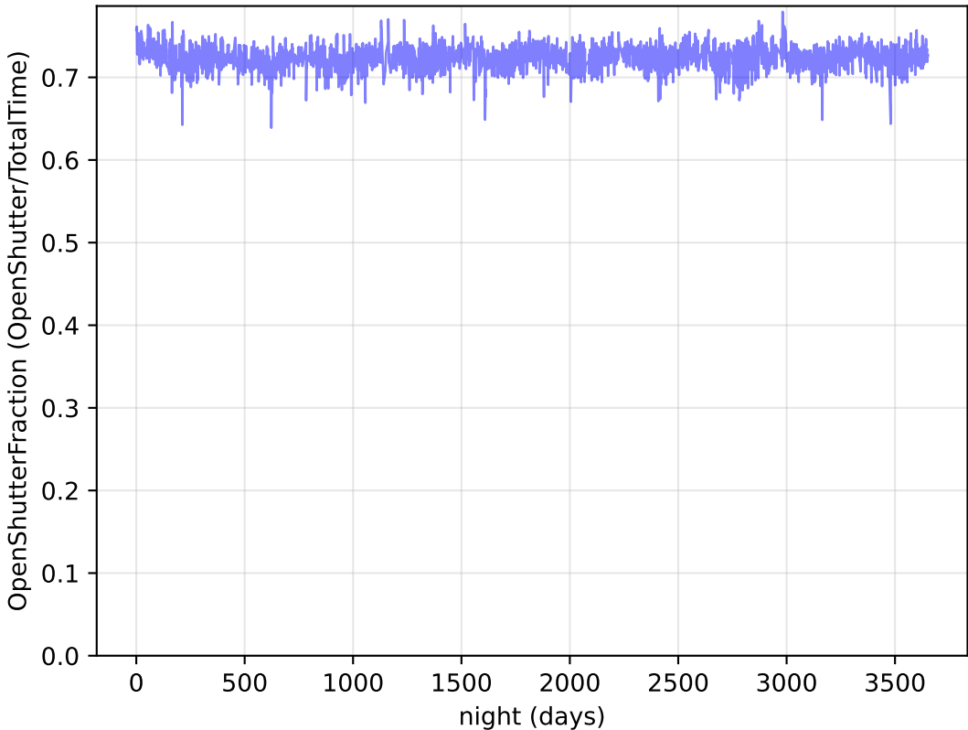
too_elab_r8_d3_giz_v3.4_10yrs Per night: OpenShutterFraction
