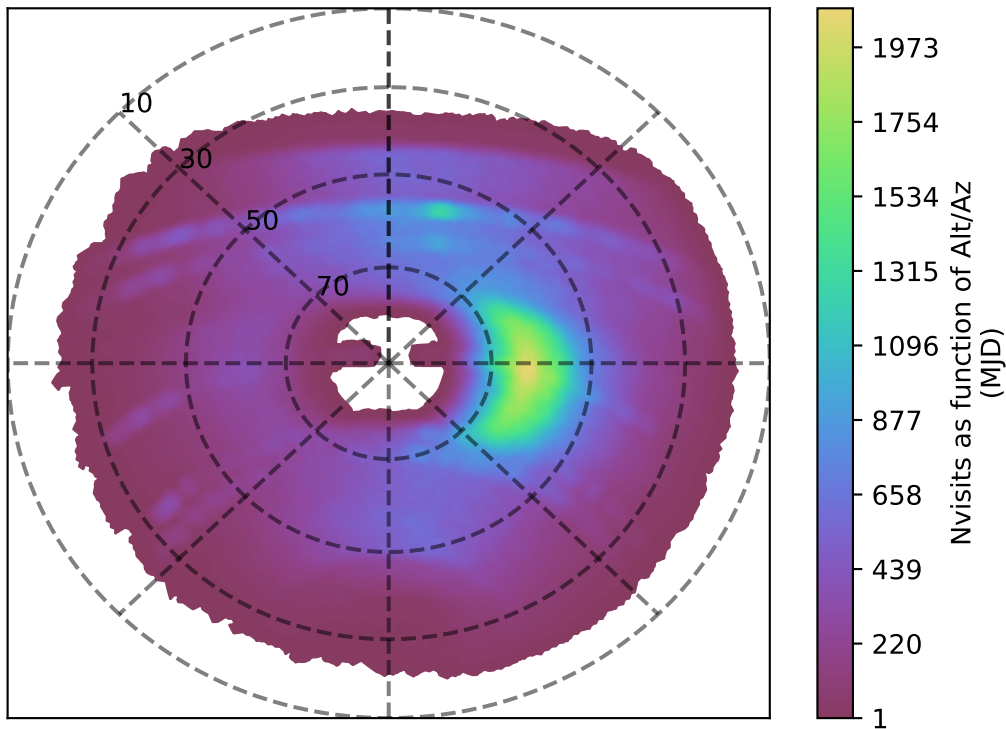
too_elab_r8_d3_giz_v3.4_10yrs y band: Nvisits as function of Alt/Az
