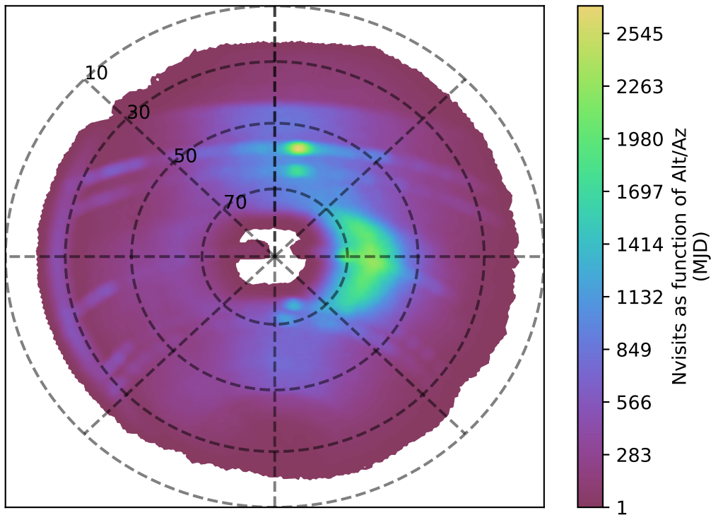
too_elab_r8_d3_giz_v3.4_10yrs r band: Nvisits as function of Alt/Az
