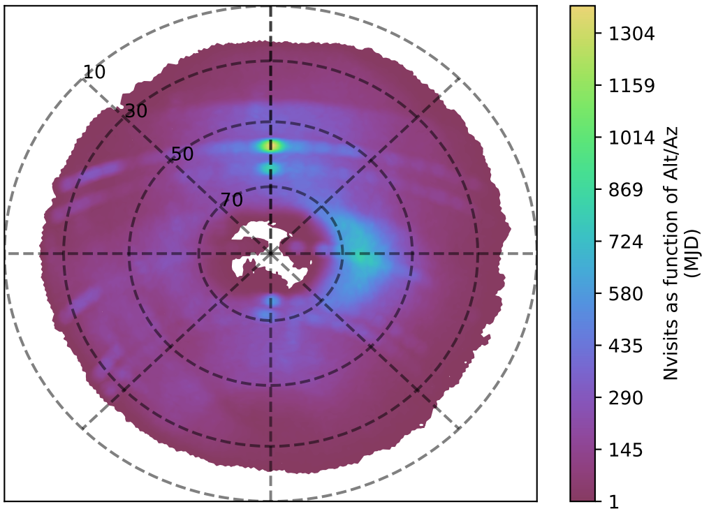
too_elab_r8_d3_giz_v3.4_10yrs g band: Nvisits as function of Alt/Az
