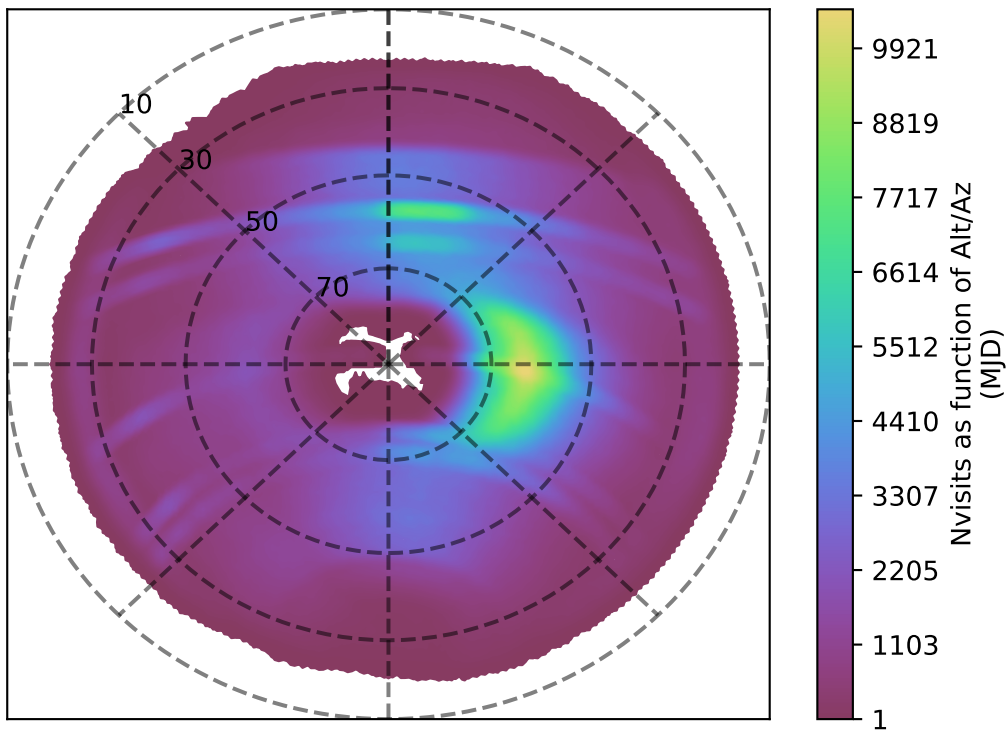
too_elab_r8_d3_giz_v3.4_10yrs all bands: Nvisits as function of Alt/Az
