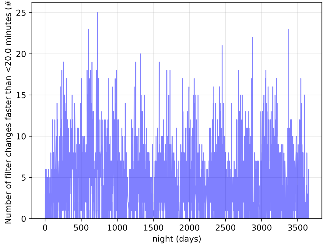
too_elab_r8_d3_giz_v3.4_10yrs Per Night: Number of filter changes faster than <20.0 minutes
