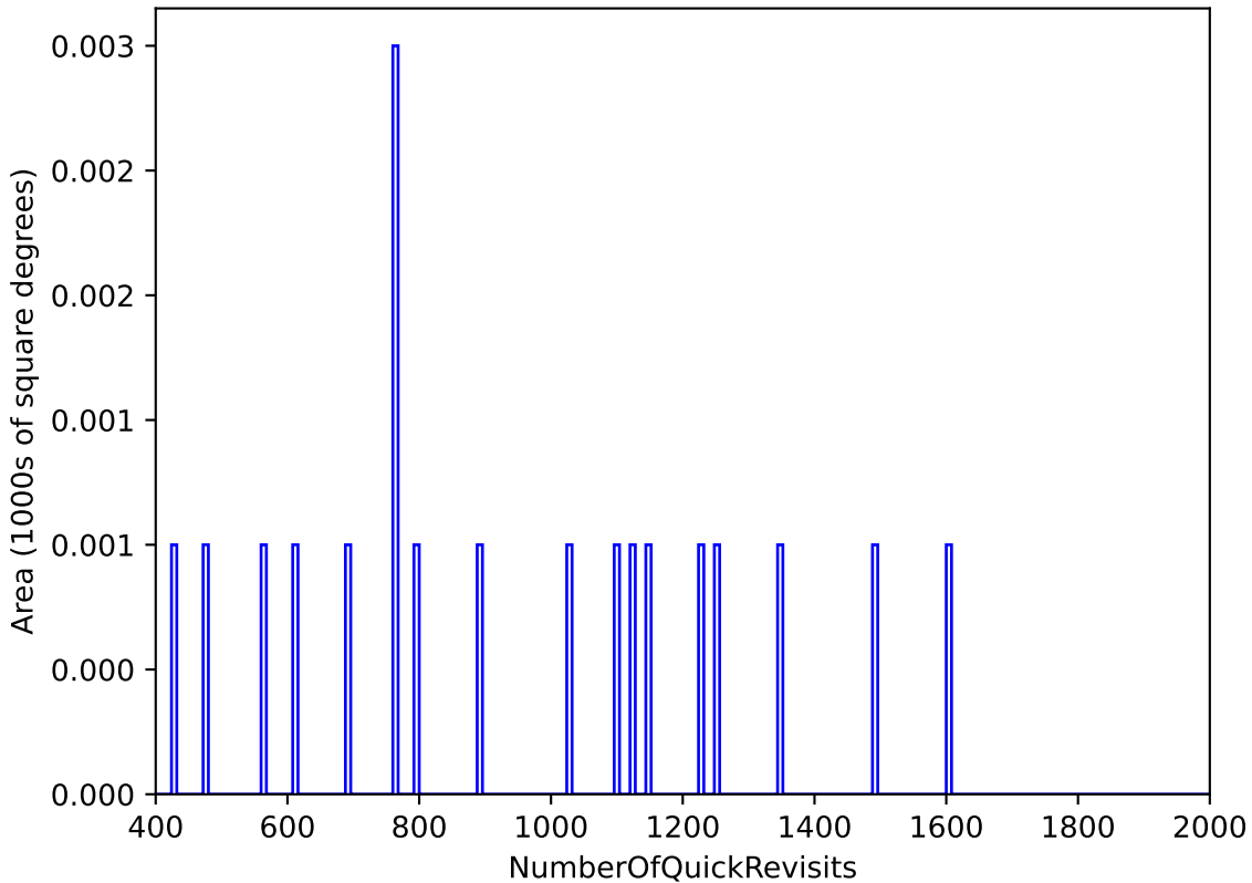
too_elab_r8_d3_giz_v3.4_10yrs All sky: NumberOfQuickRevisits
