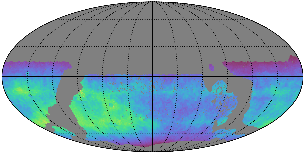
too_elab_r8_d3_giz_v3.4_10yrs WFD z band: Normalized Teff
