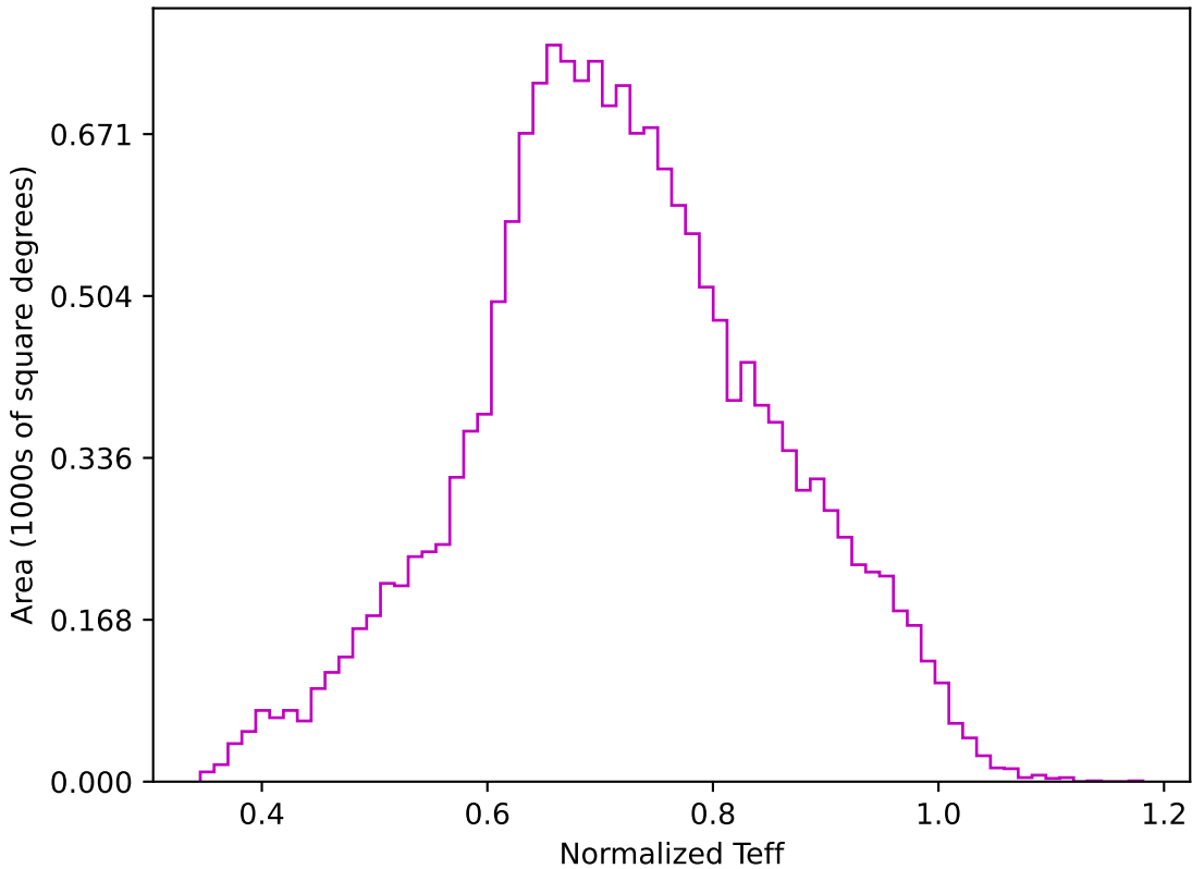
too_elab_r8_d3_giz_v3.4_10yrs WFD z band: Normalized Teff
