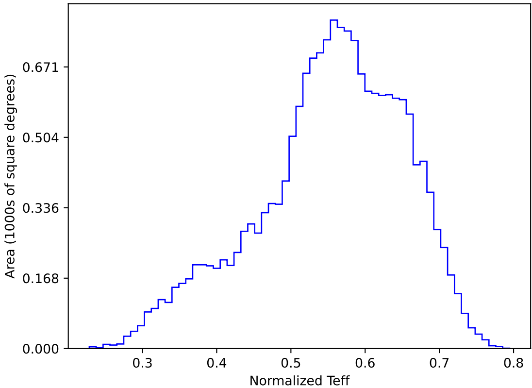
too_elab_r8_d3_giz_v3.4_10yrs WFD y band: Normalized Teff
