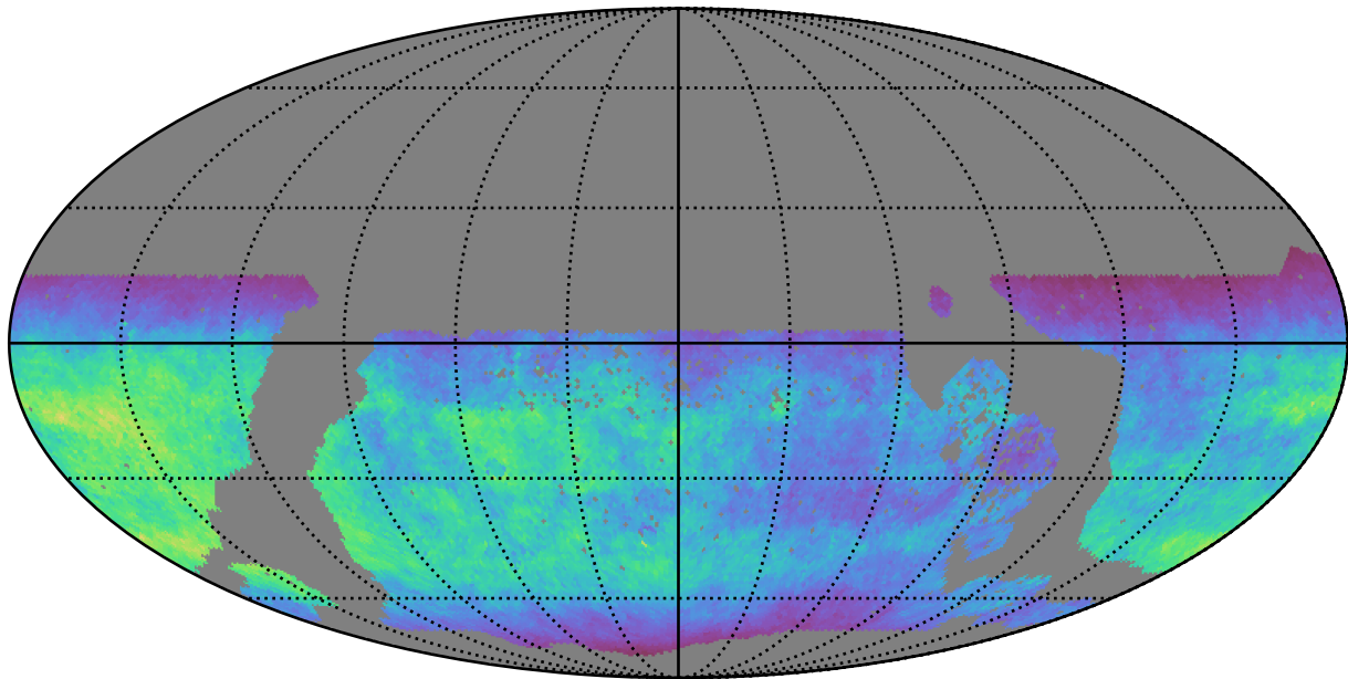
too_elab_r8_d3_giz_v3.4_10yrs WFD u band: Normalized Teff
