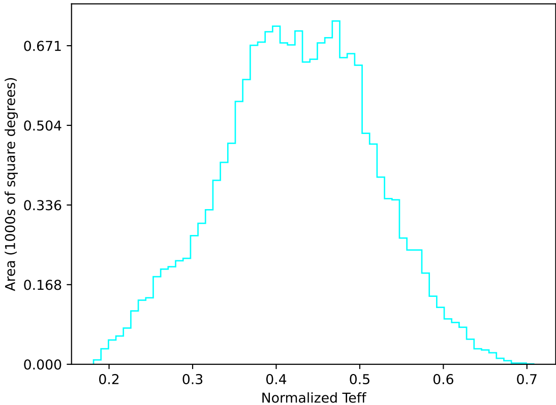
too_elab_r8_d3_giz_v3.4_10yrs WFD u band: Normalized Teff
