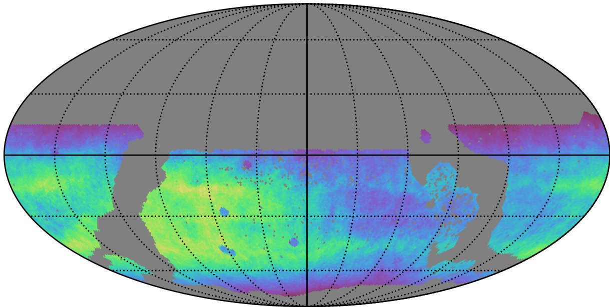
too_elab_r8_d3_giz_v3.4_10yrs WFD r band: Normalized Teff
