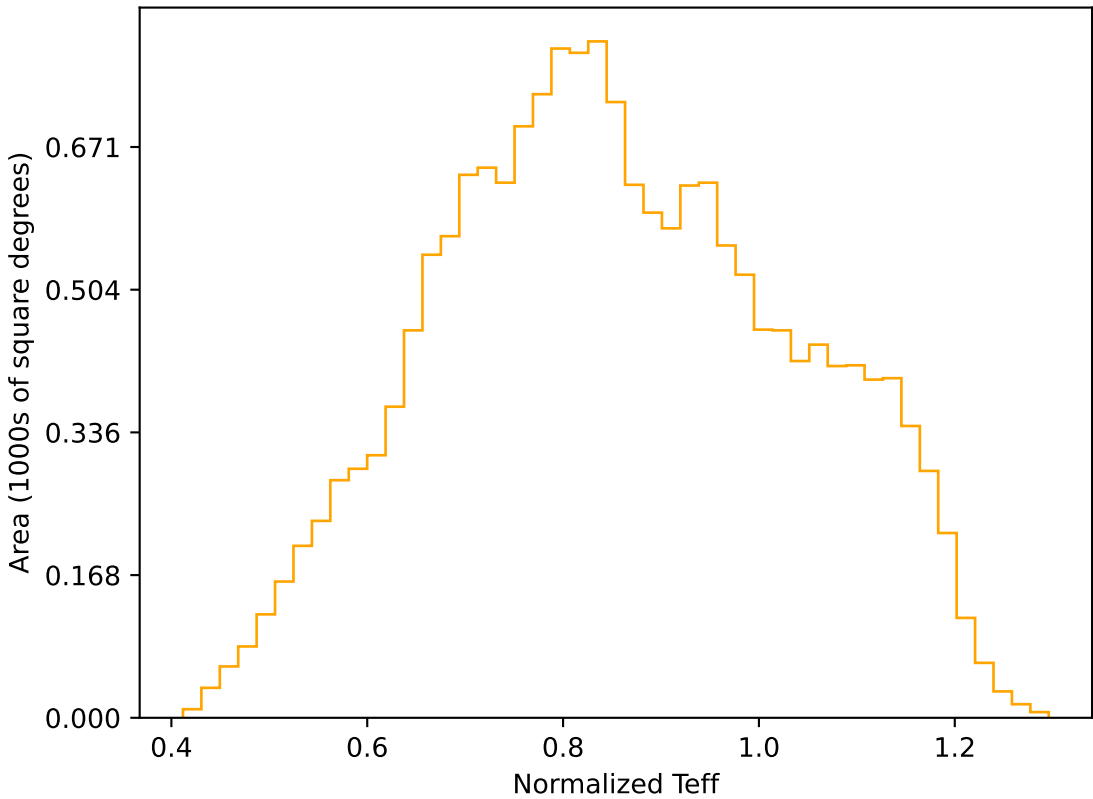
too_elab_r8_d3_giz_v3.4_10yrs WFD r band: Normalized Teff
