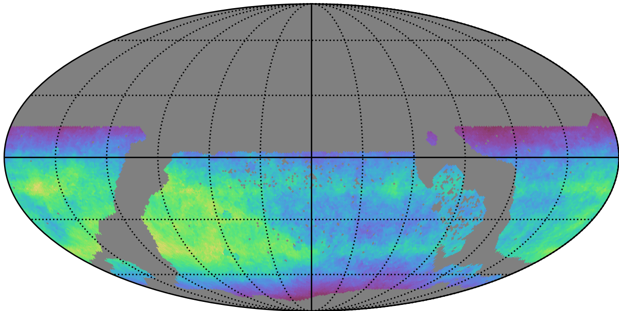
too_elab_r8_d3_giz_v3.4_10yrs WFD i band: Normalized Teff
