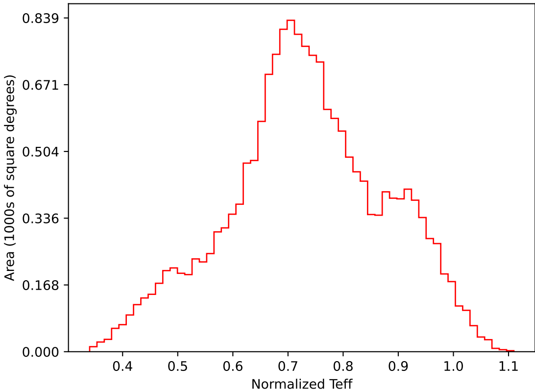
too_elab_r8_d3_giz_v3.4_10yrs WFD i band: Normalized Teff
