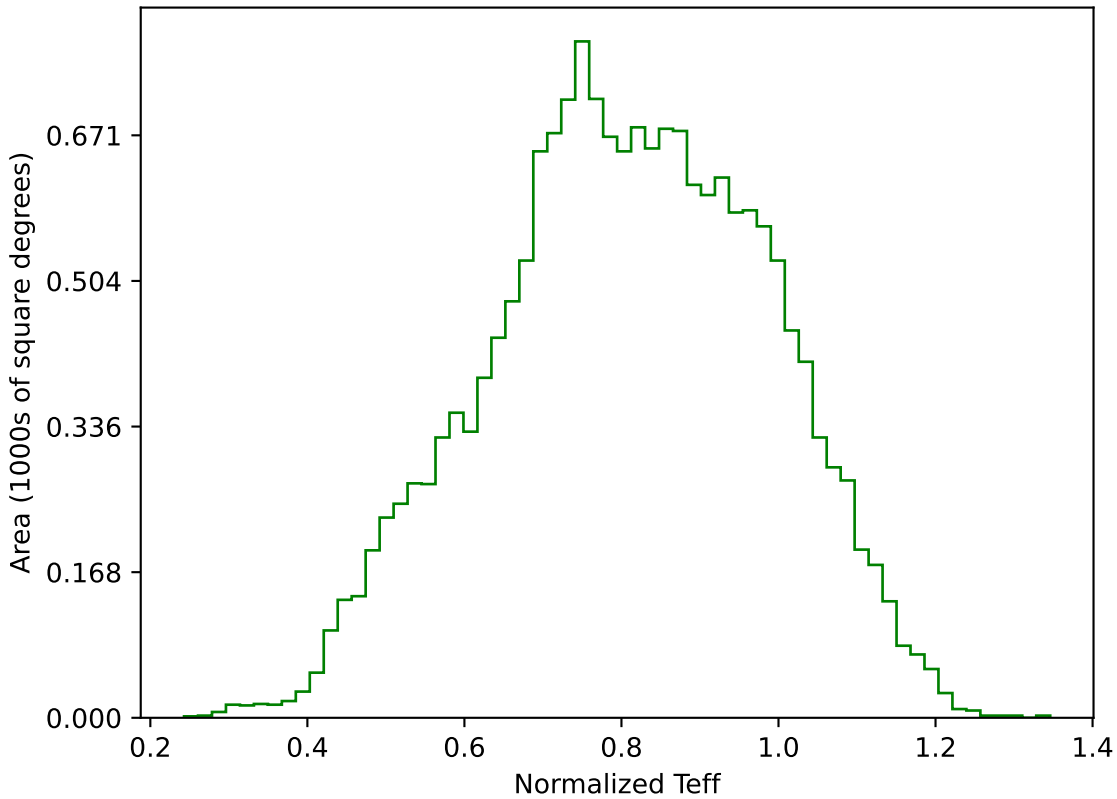
too_elab_r8_d3_giz_v3.4_10yrs WFD g band: Normalized Teff
