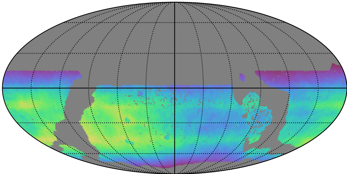
too_elab_r8_d3_giz_v3.4_10yrs WFD all bands: Normalized Teff
