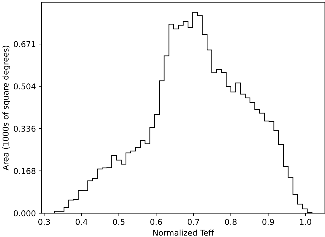
too_elab_r8_d3_giz_v3.4_10yrs WFD all bands: Normalized Teff
