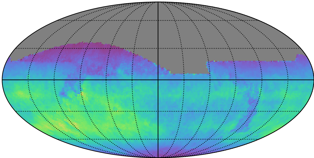
too_elab_r8_d3_giz_v3.4_10yrs All sky z band: Normalized Teff
