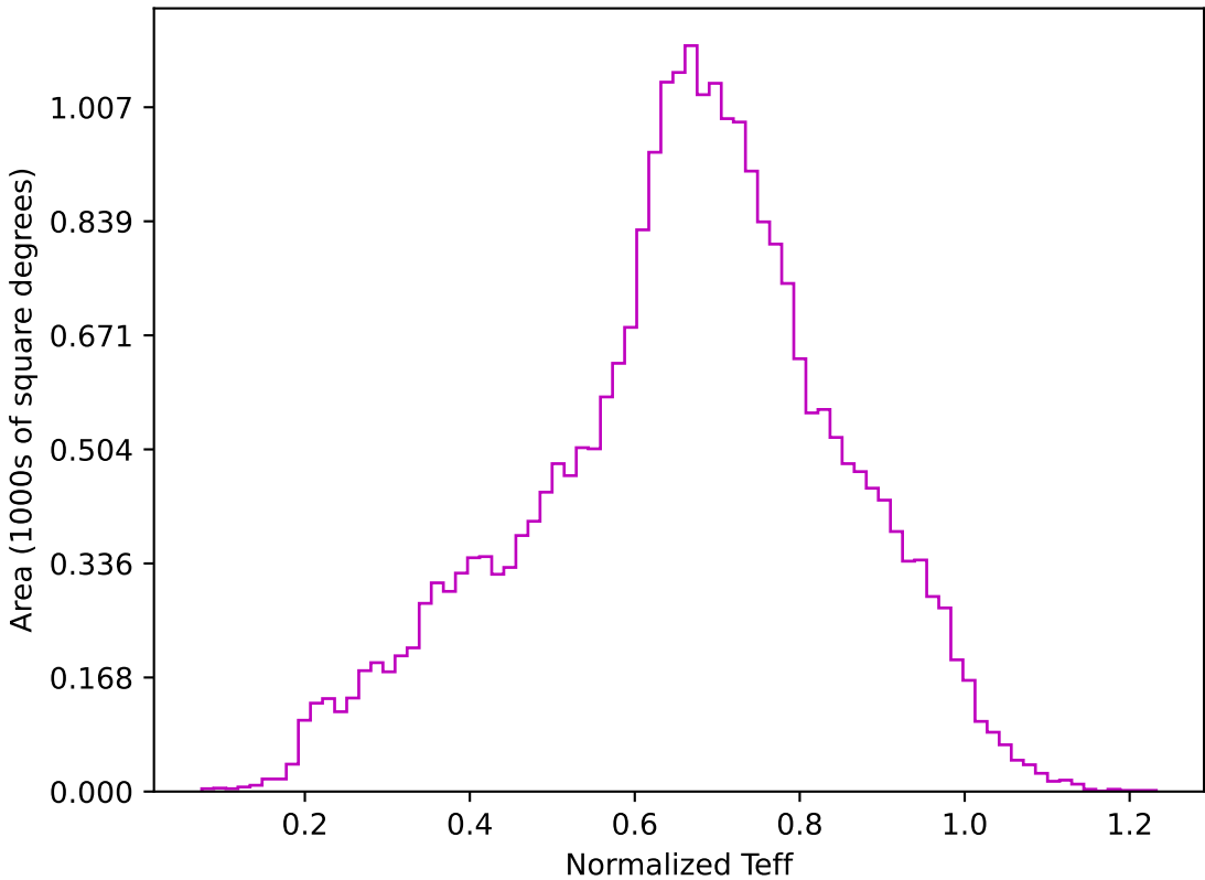
too_elab_r8_d3_giz_v3.4_10yrs All sky z band: Normalized Teff
