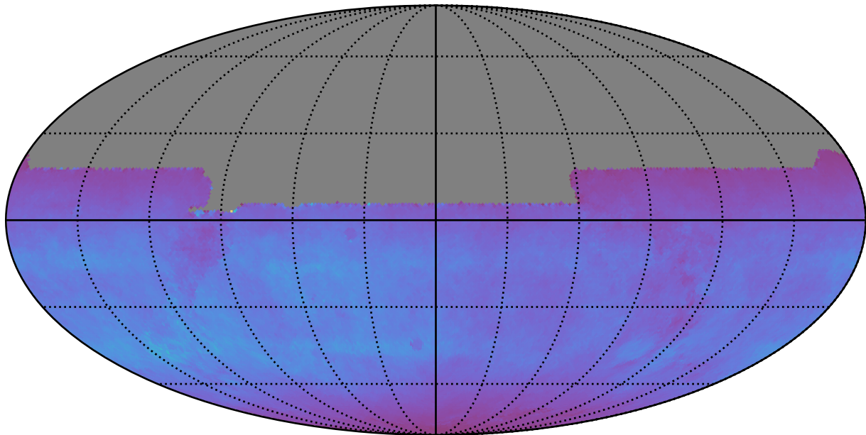
too_elab_r8_d3_giz_v3.4_10yrs All sky y band: Normalized Teff
