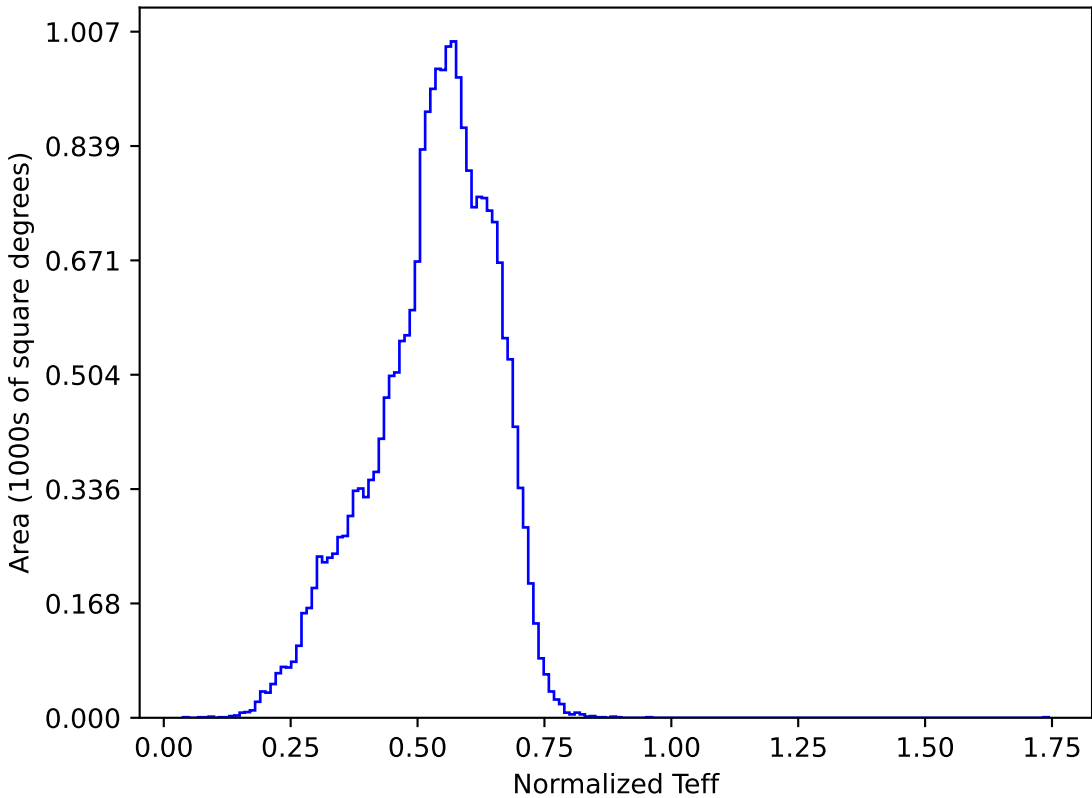
too_elab_r8_d3_giz_v3.4_10yrs All sky y band: Normalized Teff
