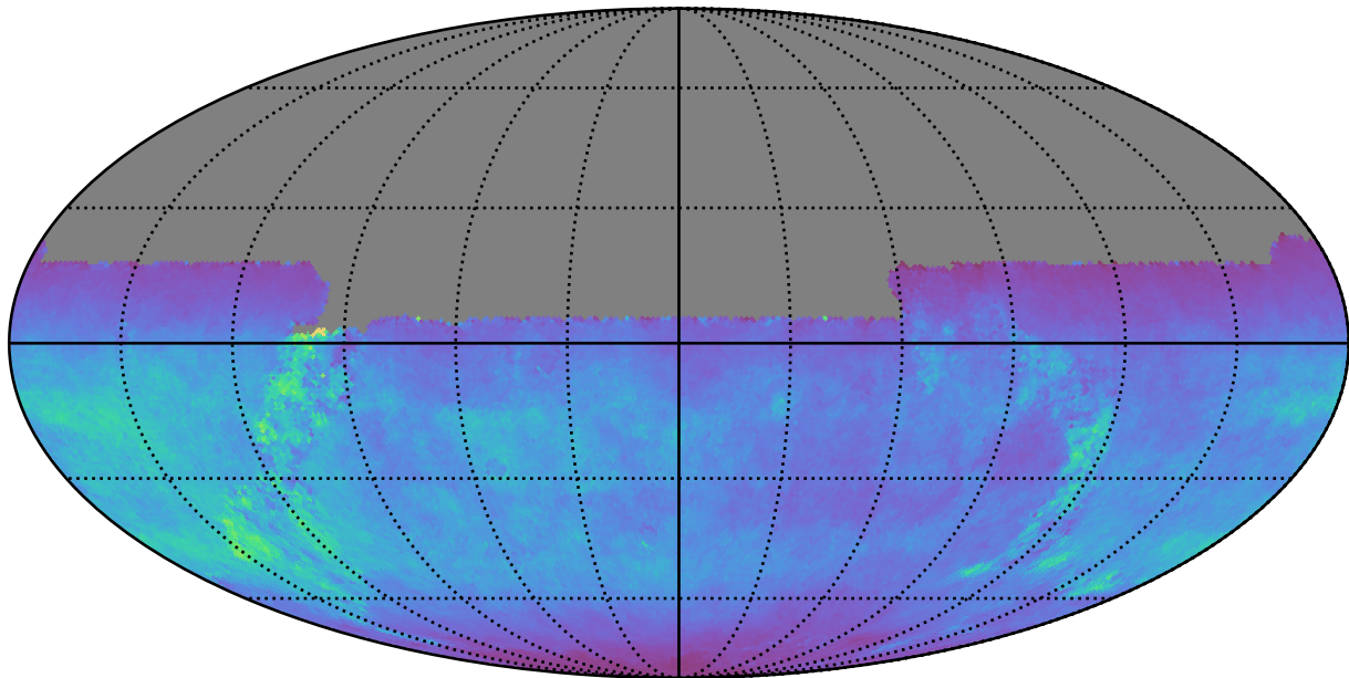
too_elab_r8_d3_giz_v3.4_10yrs All sky u band: Normalized Teff
