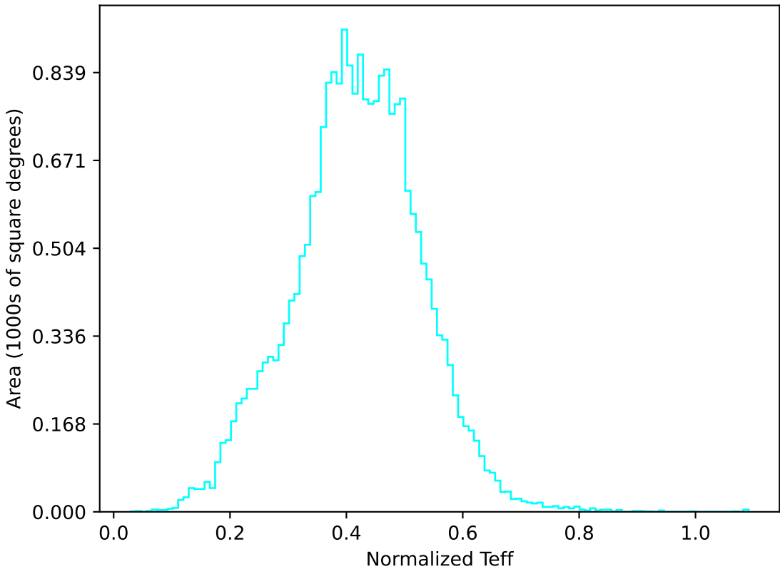
too_elab_r8_d3_giz_v3.4_10yrs All sky u band: Normalized Teff
