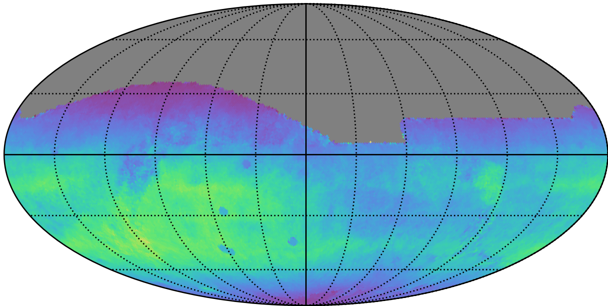
too_elab_r8_d3_giz_v3.4_10yrs All sky r band: Normalized Teff
