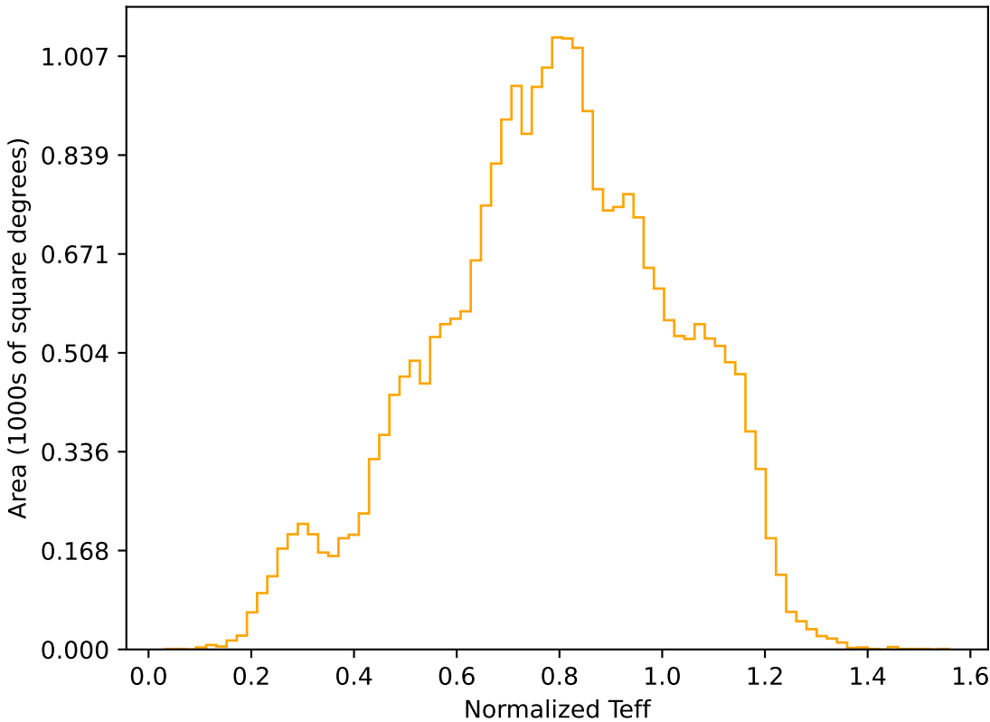
too_elab_r8_d3_giz_v3.4_10yrs All sky r band: Normalized Teff
