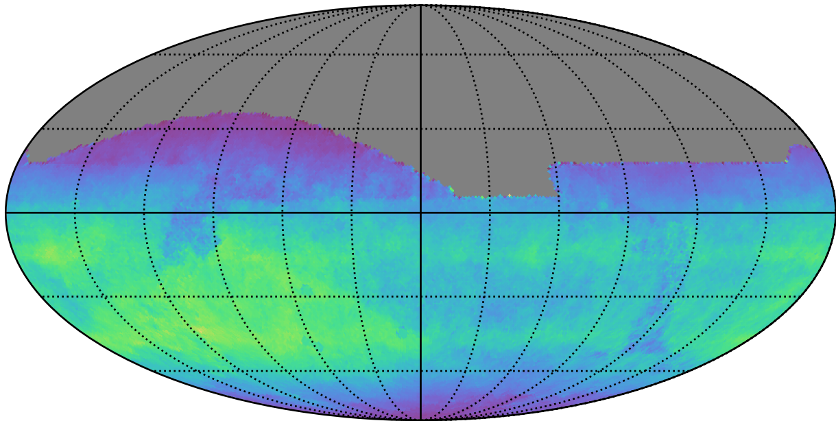
too_elab_r8_d3_giz_v3.4_10yrs All sky i band: Normalized Teff
