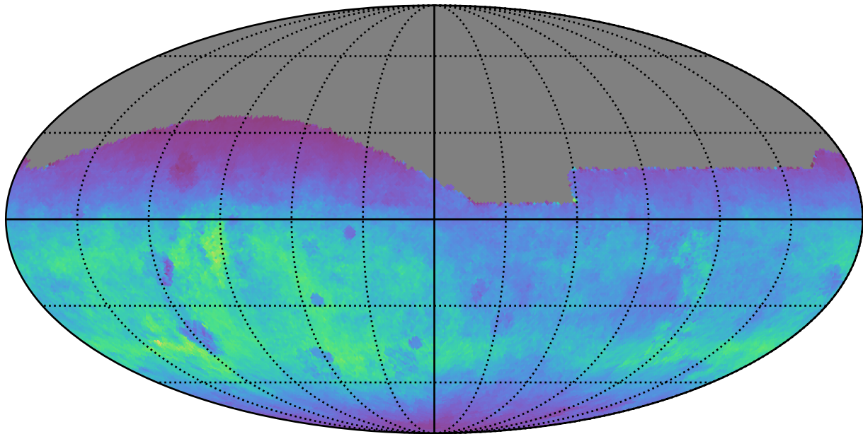
too_elab_r8_d3_giz_v3.4_10yrs All sky g band: Normalized Teff
