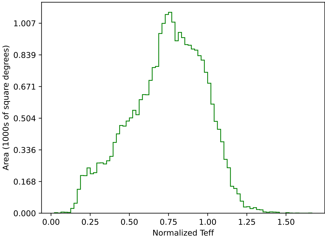
too_elab_r8_d3_giz_v3.4_10yrs All sky g band: Normalized Teff
