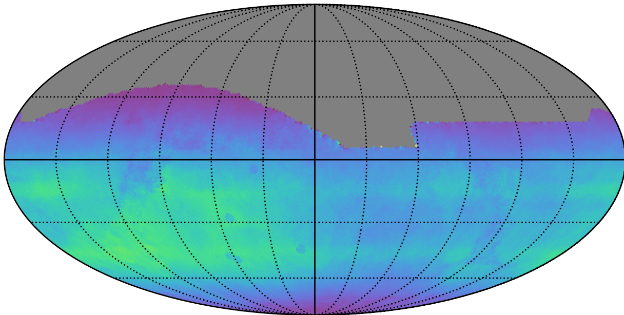
too_elab_r8_d3_giz_v3.4_10yrs All sky all bands: Normalized Teff
