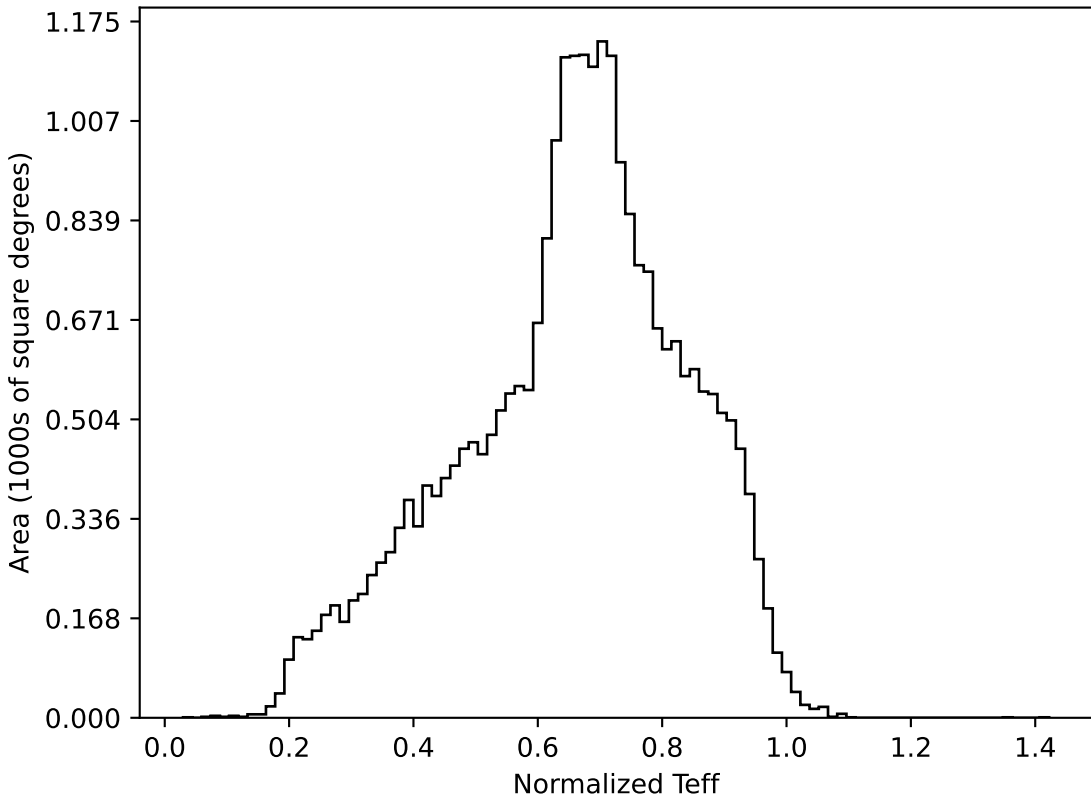
too_elab_r8_d3_giz_v3.4_10yrs All sky all bands: Normalized Teff
