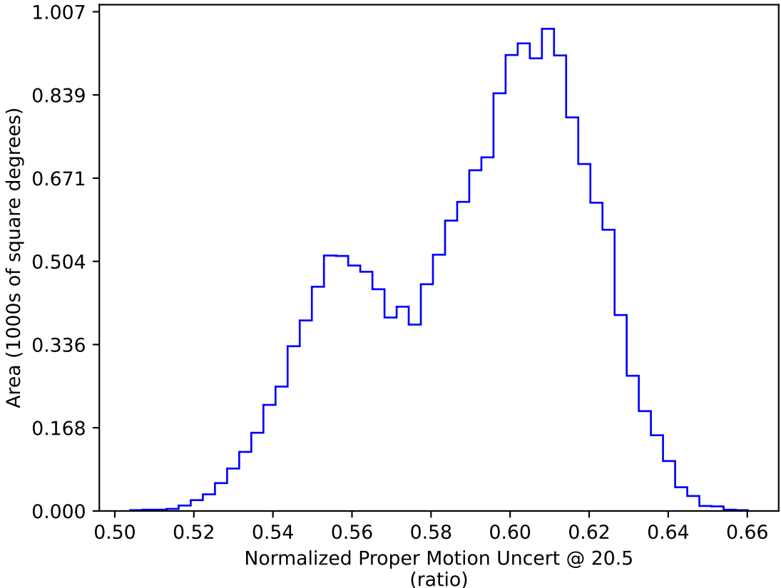
too_elab_r8_d3_giz_v3.4_10yrs WFD: Normalized Proper Motion Uncert @ 20.5
