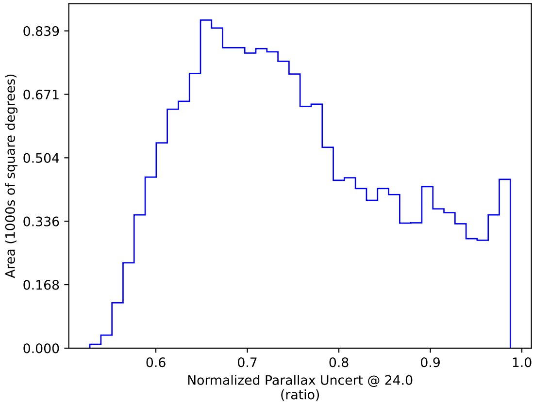
too_elab_r8_d3_giz_v3.4_10yrs WFD: Normalized Parallax Uncert @ 24.0
