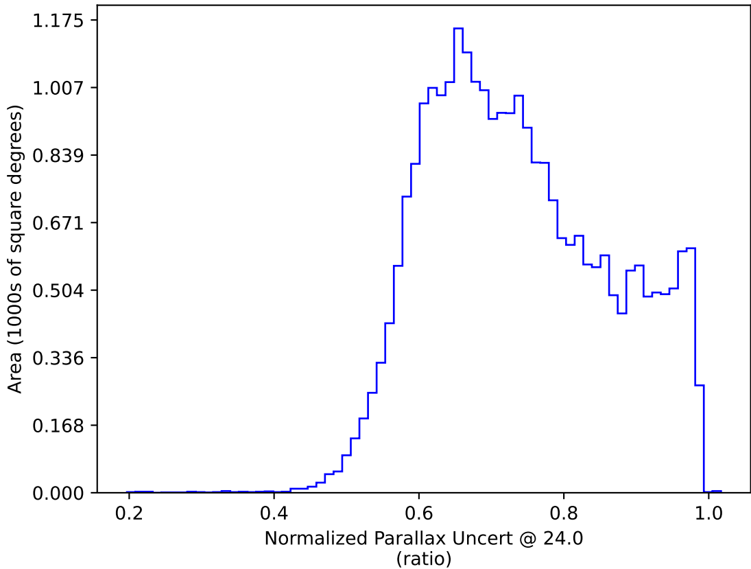
too_elab_r8_d3_giz_v3.4_10yrs All sky: Normalized Parallax Uncert @ 24.0
