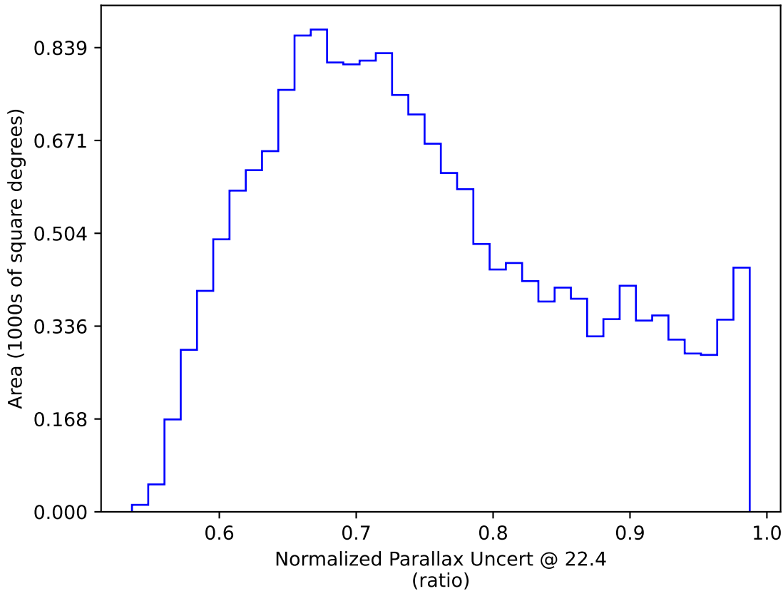
too_elab_r8_d3_giz_v3.4_10yrs WFD: Normalized Parallax Uncert @ 22.4
