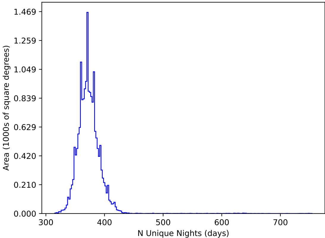
too_elab_r8_d3_giz_v3.4_10yrs WFD all bands: N Unique Nights
