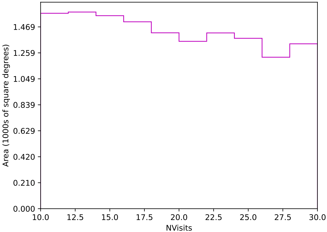
too_elab_r8_d3_giz_v3.4_10yrs Yr 3-4 z band: NVisits
