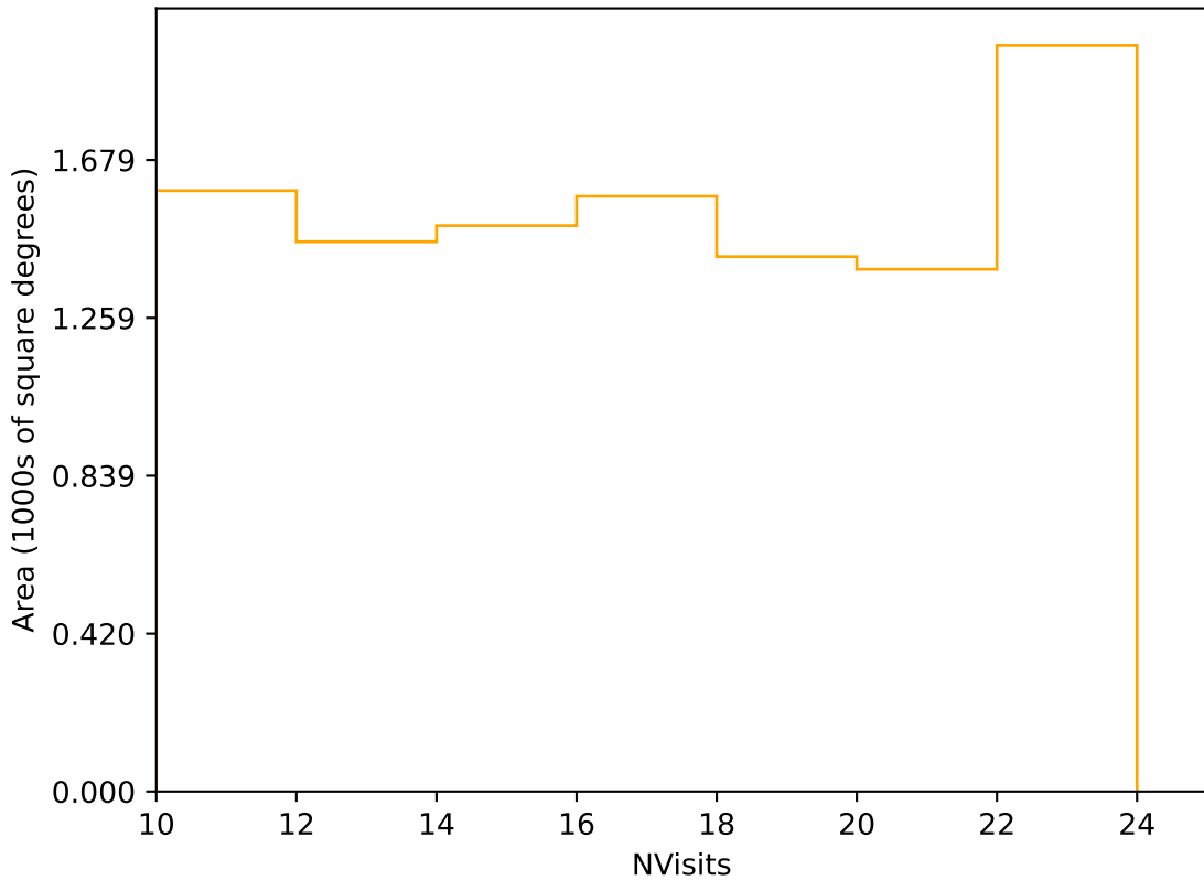
too_elab_r8_d3_giz_v3.4_10yrs Yr 3-4 r band: NVisits
