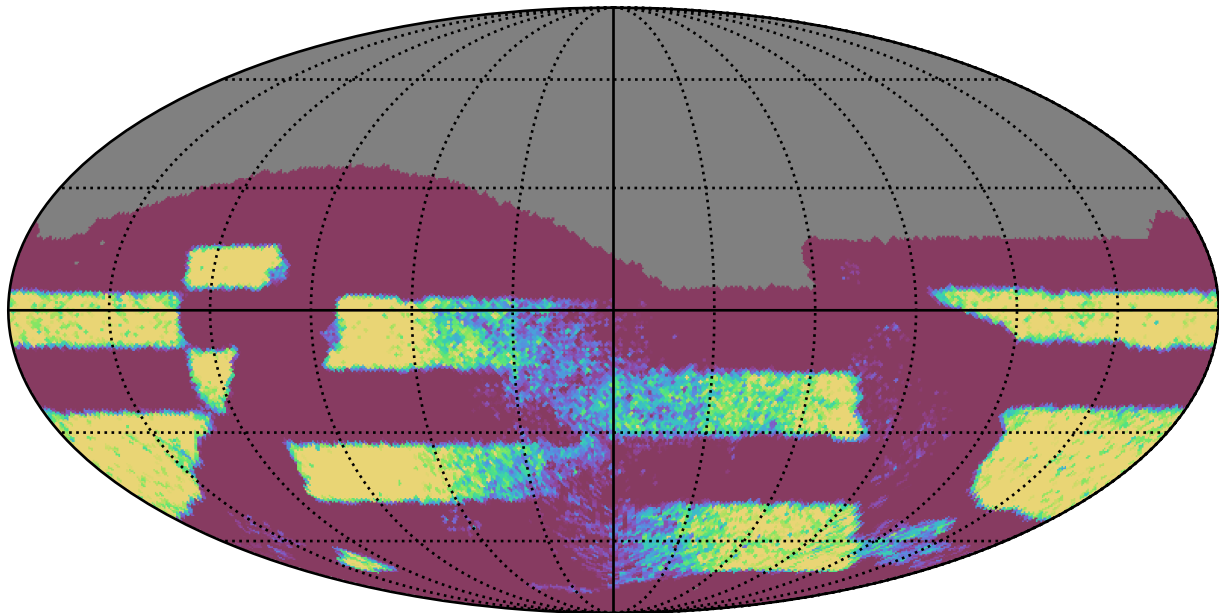
too_elab_r8_d3_giz_v3.4_10yrs Yr 3-4 all bands: NVisits
