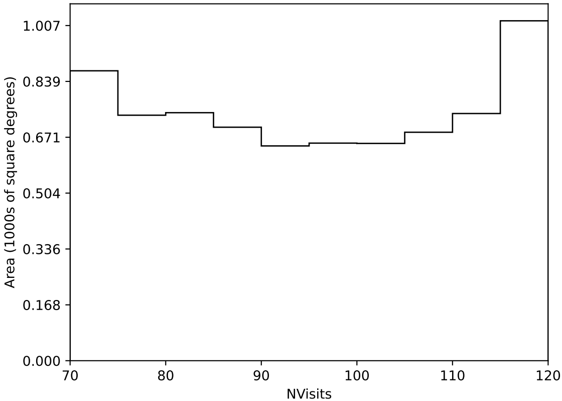
too_elab_r8_d3_giz_v3.4_10yrs Yr 3-4 all bands: NVisits
