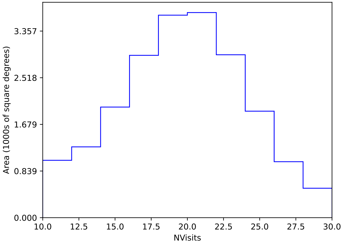
too_elab_r8_d3_giz_v3.4_10yrs Yr 1 y band: NVisits
